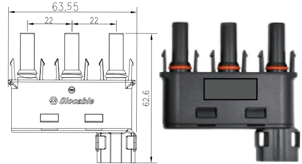
三母一公 BC50-3F1M 3 Female to 1 Male
