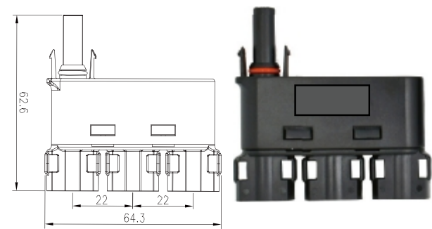
三公一母 BC50-3M1F 3 Male to 1 Female
