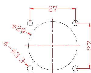
Panel cutout
