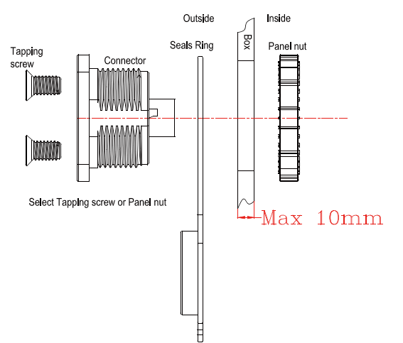
Installation method
